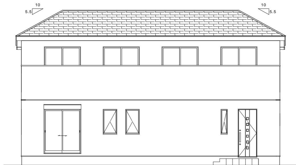
南 SouthFacing Elevation
